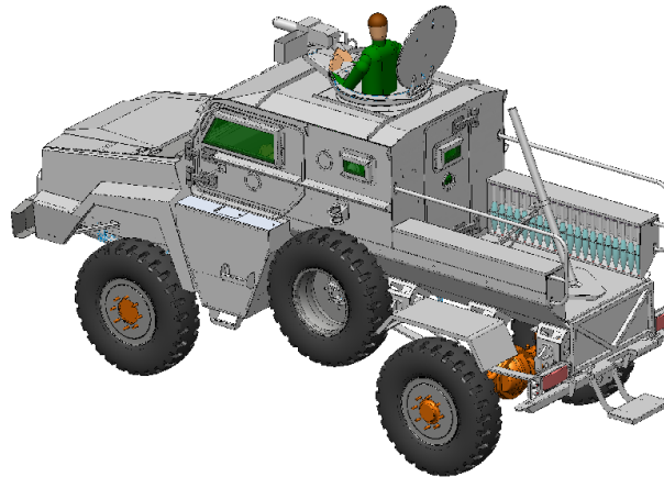
60mm Mortar and 40mm AGL carrier
